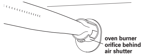
L.P. oven orifice spud stamped with "56"
