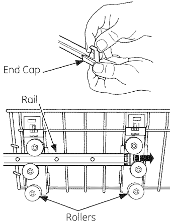
Upper Rack - 8 Place Settings - GDF510 & GDF520
