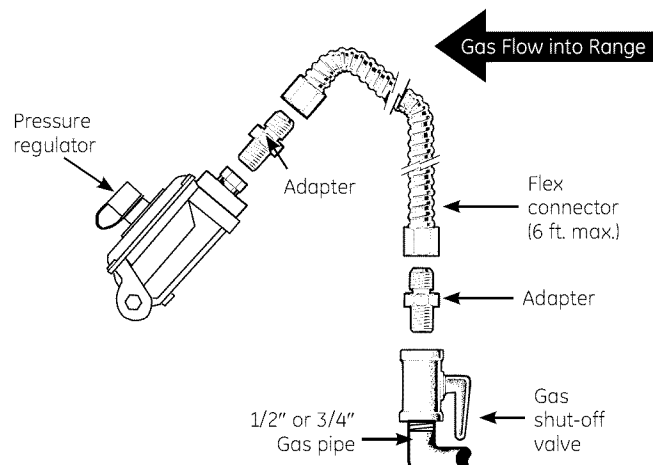
Gasline from wall
