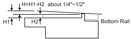
Vinyl-Clad Window
