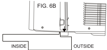
Vinyl-Clad Windows
