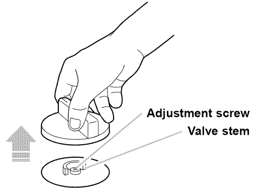
Low flame
